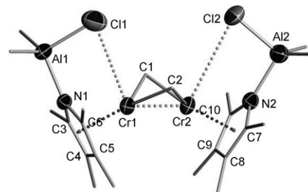
Figure 2. Plot of 3 with ellipsoids set at 50% probability and hydrogen atoms omitted for clarity. Selected bond lengths [Å] and angles [°]: Cl1–Al1 2.187(3), Cr1–C1 2.181(5), Cr1–C2 2.198(5), Cr2–C1 2.172(4), Cr2–C2 2.180(5), Cr1–C3 2.306(5), Cr1–C4 2.341(5), Cr1–Cr2 2.274(1), Cr1–C5 2.339(5), Cr1–C6 2.317(4), Cr1–N1 2.350(4), Al1–N1 1.984(4), Cr1–C11 3.489(8), Cr2–Cl2 3.675(8), Cr1–centroid1 2.003(5), Cr2–centroid2 1.992(5); Cr2–Cr1–centroid1 152.9(3), Cr1–Cr2–centroid2 152.9(3).
