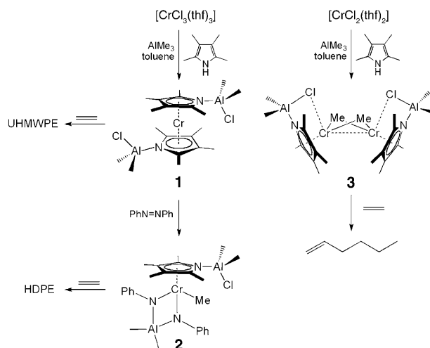
Scheme 1. Formation of complexes 1 and 2 from \text{Cr}^{\text{III}} (polymerization of ethylene to ultrahigh molecular weight PE: M_w = 2\,600\,000 , \text{PDI} = 1.7 , 45\text{ tonnes mol}^{-1} ) and 3 from \text{Cr}^{\text{II}} (generation of 1-hexene).
